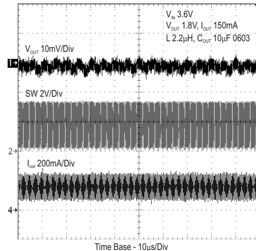
Figure 18. Typical Operation vs PWM Mode
