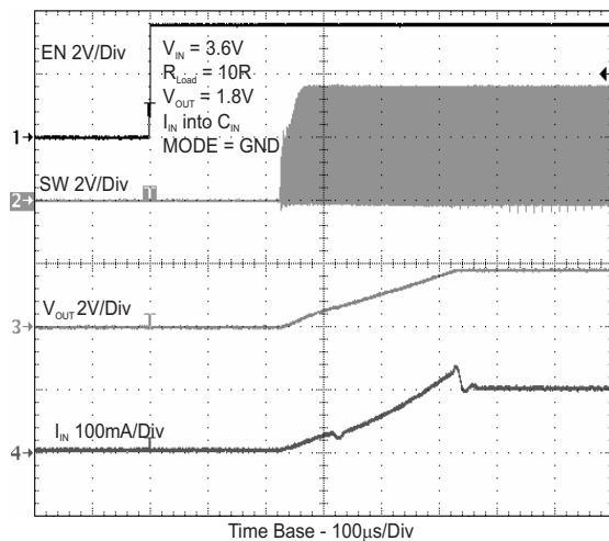
Figure 17. Start-Up Timing
