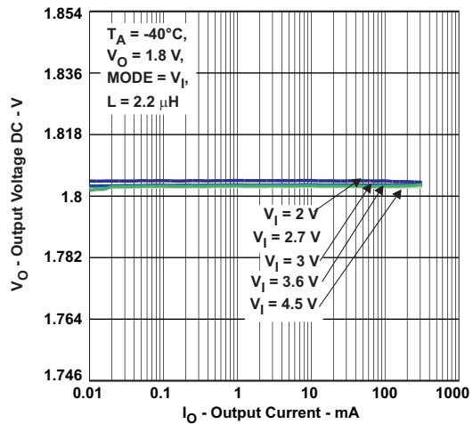
Figure 16. Output Voltage Accuracy vs Output Current
