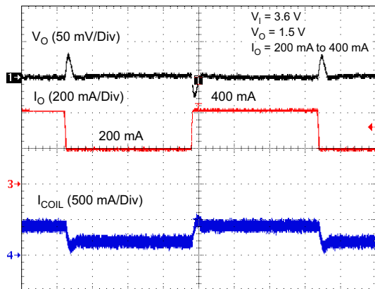
Time Base (20 \mu s/Div) Figure 25. Load Transient (Forced PWM Mode)
