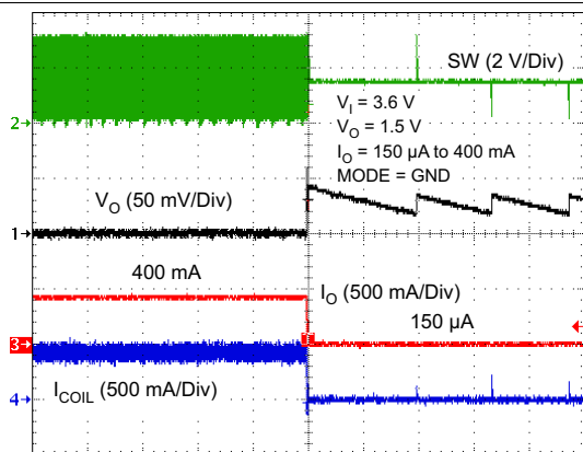
Time Base (500 \mu s/Div) Figure 27. Load Transient (PWM Mode to PFM Mode)
