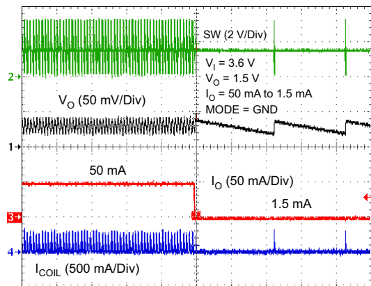
Time Base (50 \mu s/Div) Figure 29. Load Transient (PFM Mode)
