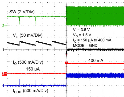
Time Base (500 \mu s/Div) Figure 26. Load Transient (PFM Mode to PWM Mode)
