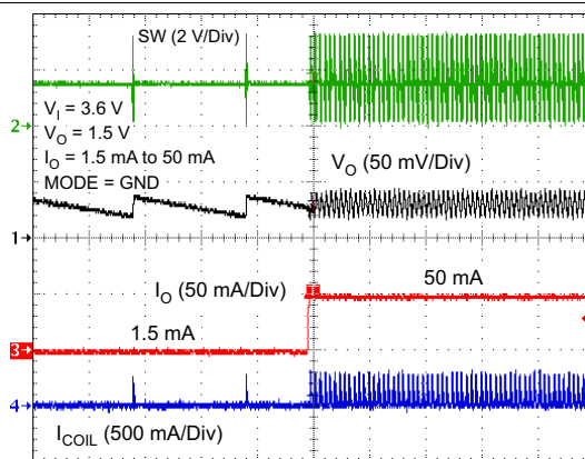
Time Base (50 \mu s/Div) Figure 28. Load Transient (PFM Mode)
