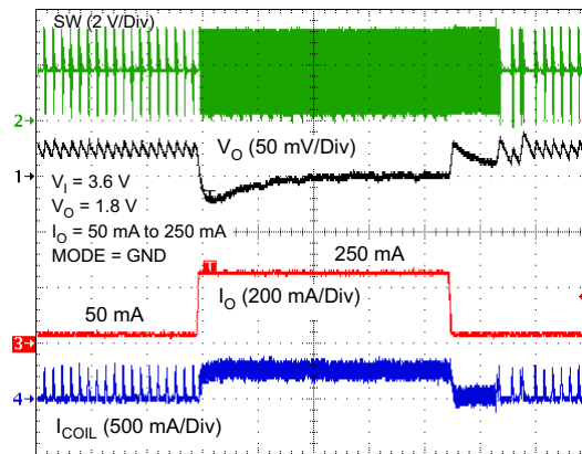
Time Base (20 \mu s/Div) Figure 30. Load Transient (PFM Mode to PWM Mode)
