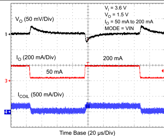
Figure 24. Load Transient (Forced PWM Mode)
