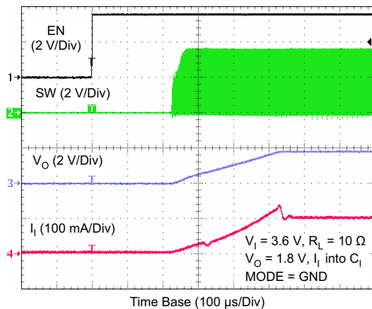
Figure 23. Start-Up Timing
