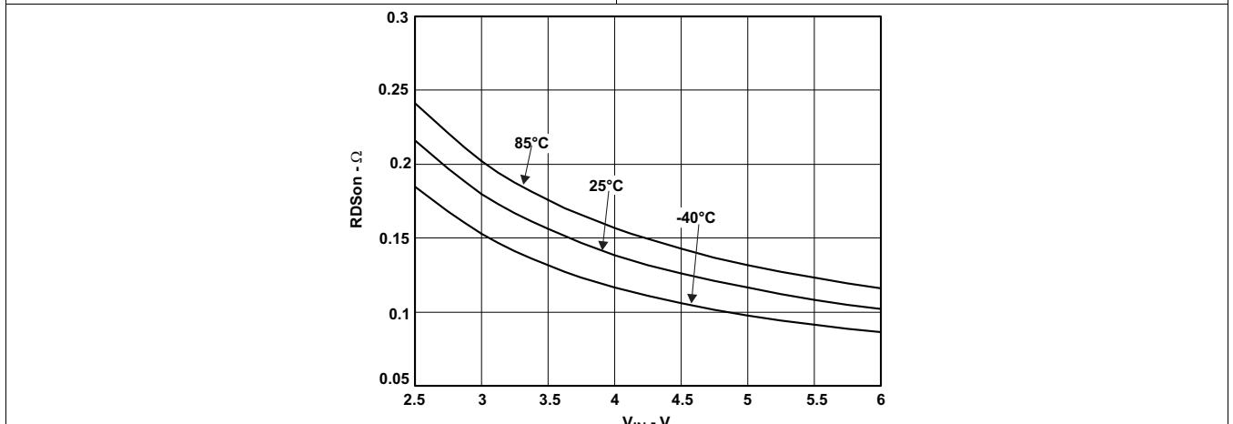
Figure 5. RDSON NMOS vs VIN
