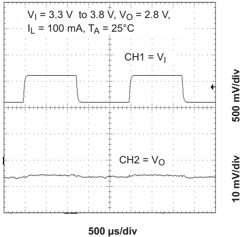
Figure 13. Line Transient Response (LDO1)
