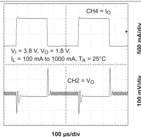
Figure 16. Load Transient Response (MAIN)
