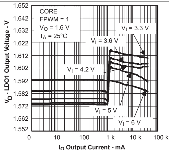
Figure 8. LD01 Output Voltage vs Output Current
