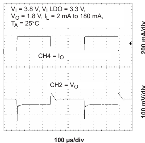
Figure 18. Load Transient Response (LDO2)
