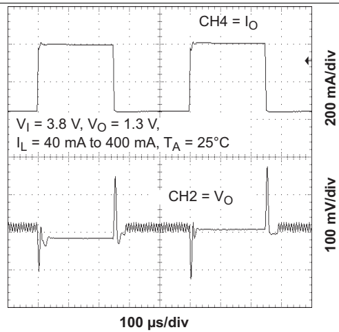
Figure 15. Load Transient Response (CORE)
