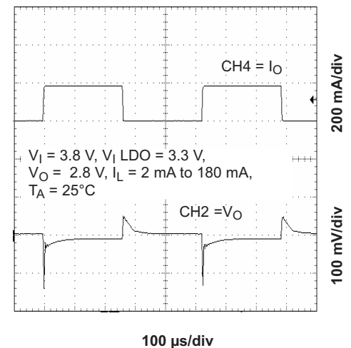
Figure 17. Load Transient Response (LDO1)
