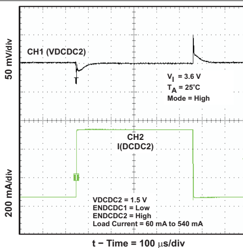
Figure 25. DCDC2 Load Transient Response
