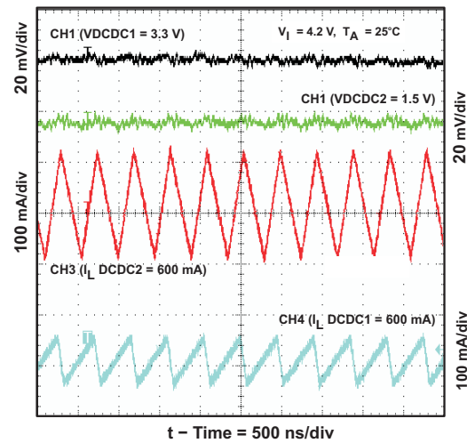
Figure 20. Output Voltage Ripple PWM Mode = HIGH
