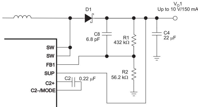
Figure 5. Feed-forward Capacitor
