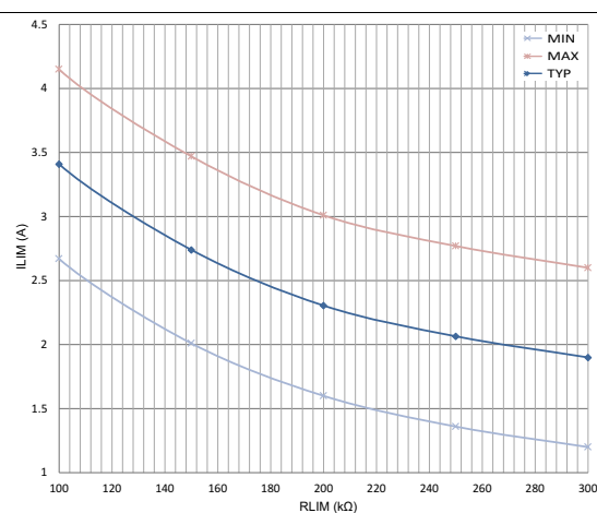
Figure 12. Current Limit V_{IN} = 12\text{ V} , f_{SW} = 500\text{ kHz}
