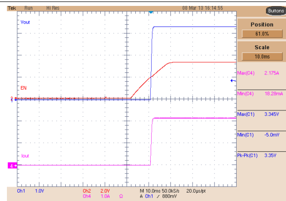
Figure 58. Buck 2 Current Limit Operation
