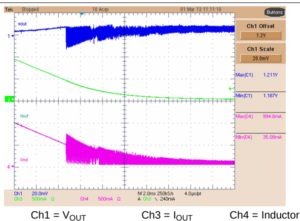
Figure 41. Buck 1 Low-Power Output, No Load
