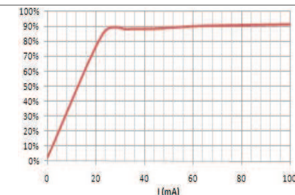
Figure 8. BUCK3 Efficiency Low-Power Enabled
