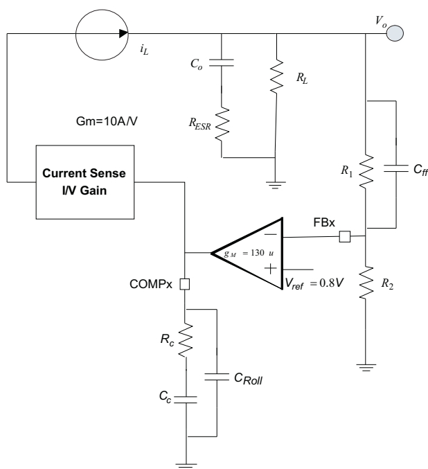
Figure 22. Loop Compensation
