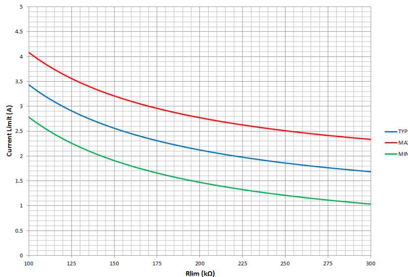
Figure 18. Buck 2
