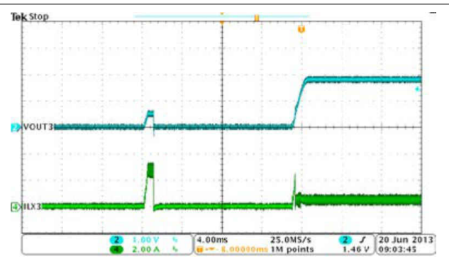
Figure 8-26. BUCK3, Hiccup and Recovery
