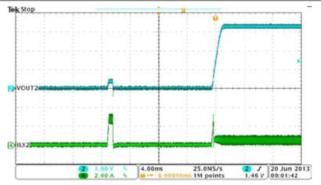
Figure 8-24. BUCK2, Hiccup and Recovery
