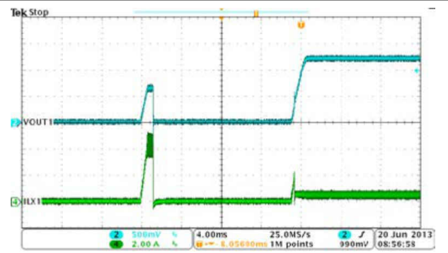
Figure 8-22. BUCK1, Hiccup and Recovery
