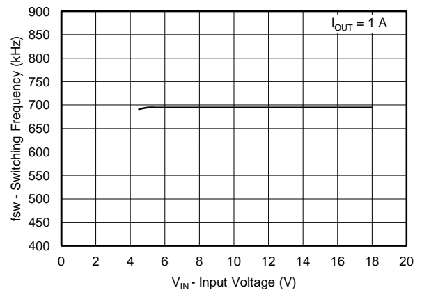
Figure 21. V OUT2 = 1.2V Switching Frequency vs Input Voltage
