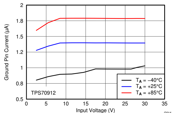
GND Current vs V_{IN} and Temperature
