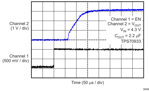
Figure 6-33. Power-Up With Enable
