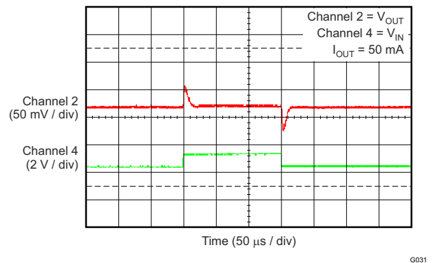
Figure 6-32. TPS70933 Line Transient (4.3 V to 5.3 V)
