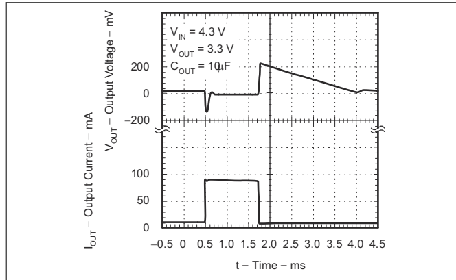
Figure 7-10. Load Transient Response (Legacy Chip)
