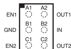
TPS718Axx, TPS719Axx YZC Package 6-BALL WCSP (Top View)
