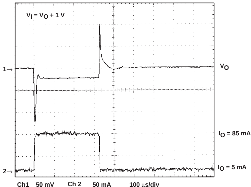
Figure 32. Load Transient Response (CSR total = 1.7 \Omega ), TPS7248Q
