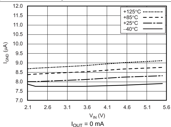
Figure 8. Ground Pin Current vs Input Voltage (TPS72718)
