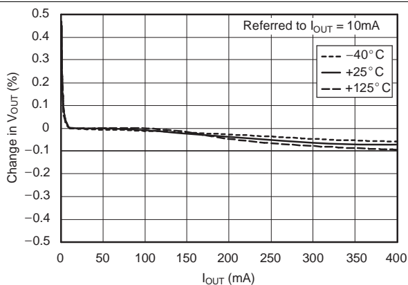
Figure 1. Load Regulation
