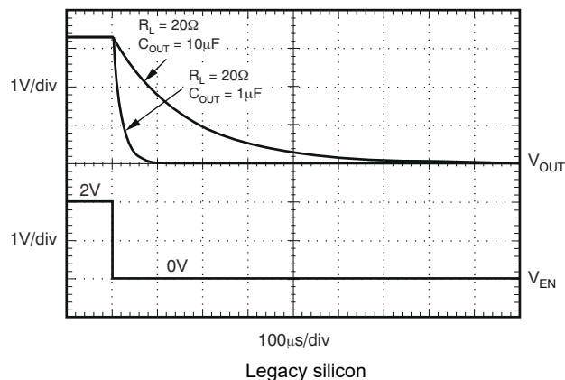
Figure 5-34. TPS73701 Turn-Off Response
