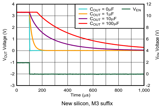
Figure 5-35. TPS73701 Turn-Off Response
