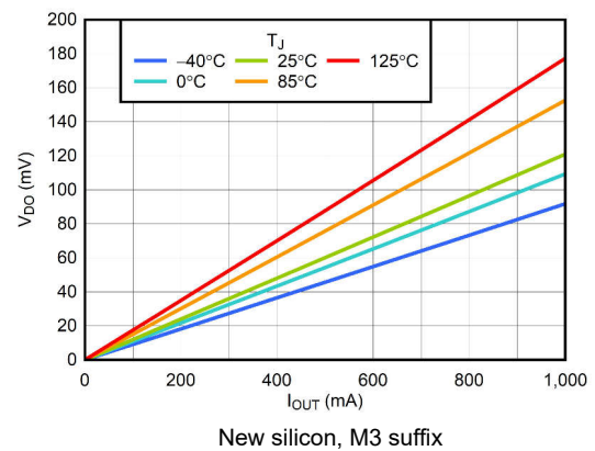
Figure 5-6. Dropout Voltage vs Output Current
