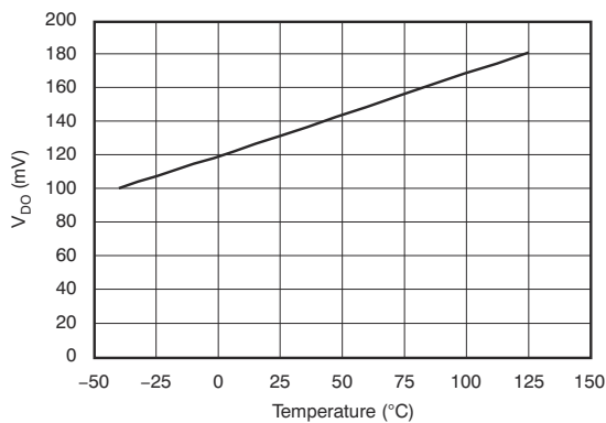
Figure 5-7. Dropout Voltage vs Temperature
