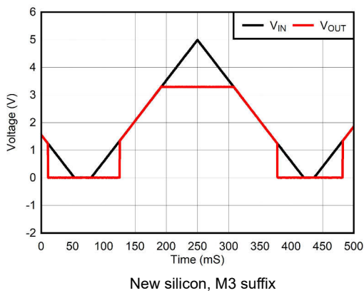
Figure 5-37. TPS73701, V_{OUT} = 3.3\text{-V} Power-Up and Power-Down
