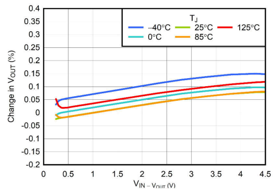
Figure 5-4. Line Regulation
