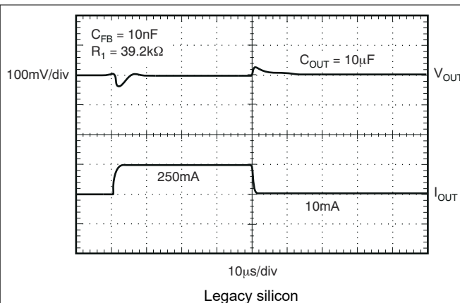
Figure 5-41. TPS73701 Load Transient, Adjustable Version
