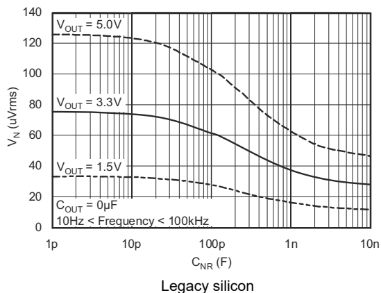
Figure 5-29. RMS Noise Voltage vs C_{NR}
