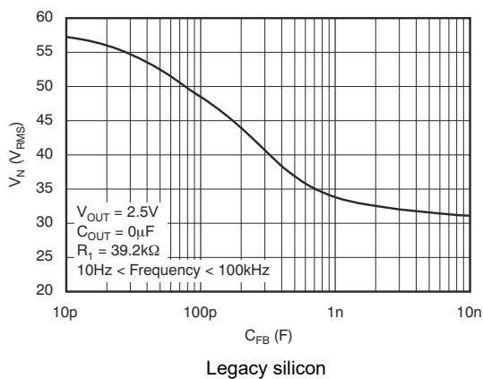
Figure 5-39. TPS73701 RMS Noise Voltage vs C_{FB}
