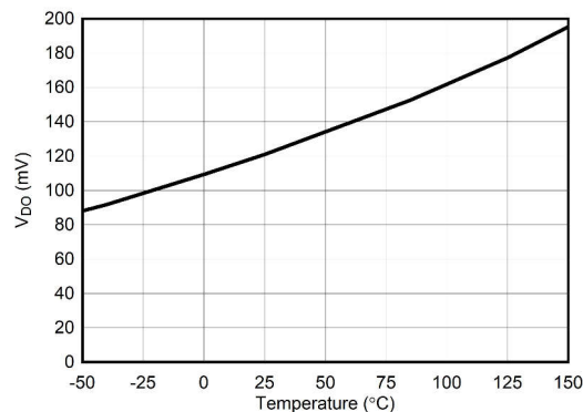
Figure 5-8. Dropout Voltage vs Temperature
