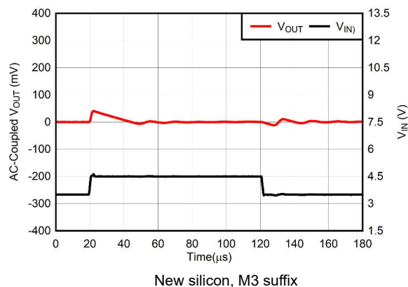
Figure 5-43. TPS73701 Line Transient, Adjustable Version
