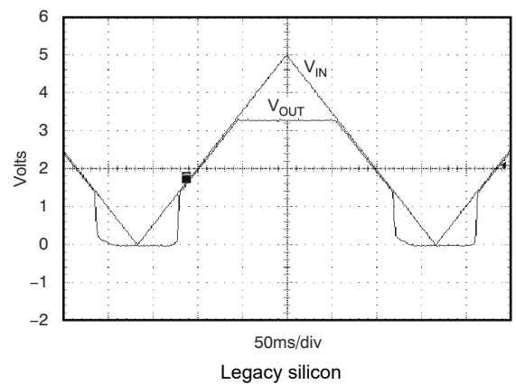
Figure 5-36. TPS73701, V_{OUT} = 3.3\text{-V} Power-Up and Power-Down
