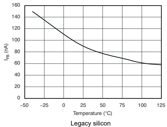
Figure 5-40. TPS73701 I_{FB} vs Temperature
