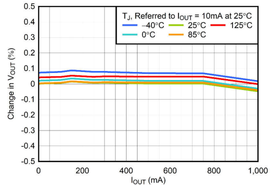
Figure 5-2. Load Regulation
