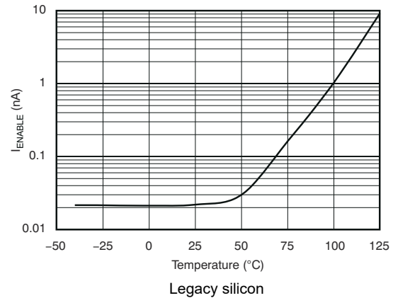
Figure 5-38. I_{EN} vs Temperature
