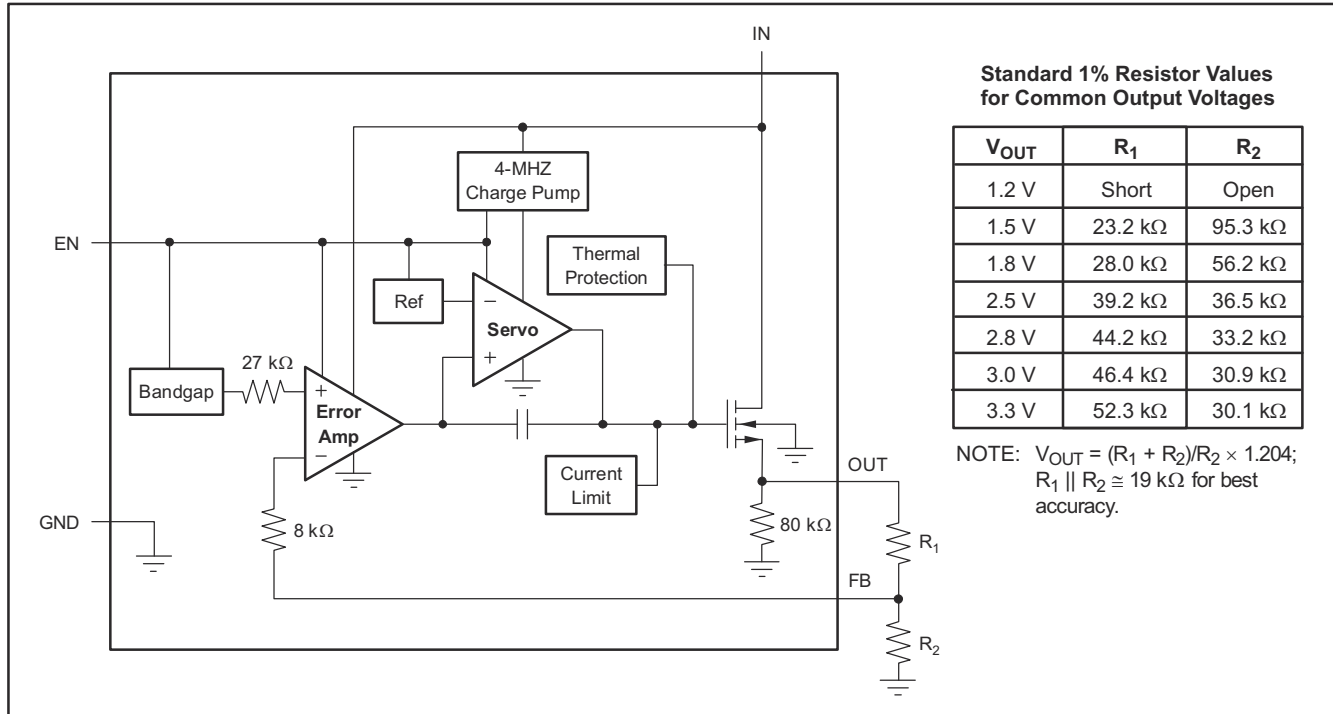
Figure 6-2. Adjustable-Voltage Version
