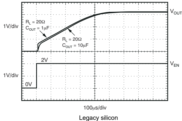
Figure 5-32. TPS73701 Turn-On Response
