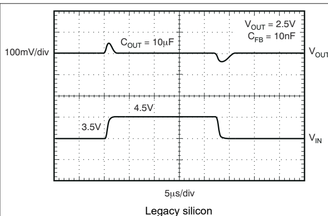
Figure 5-42. TPS73701 Line Transient, Adjustable Version
