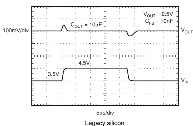
Figure 5-42. TPS73701 Line Transient, Adjustable Version
