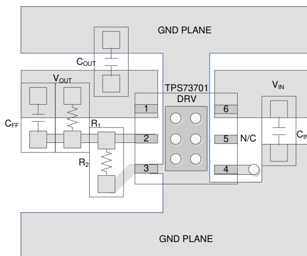
Figure 7-9. Layout Example
