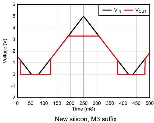
Figure 5-37. TPS73701, V_{OUT} = 3.3\text{-V} Power-Up and Power-Down
