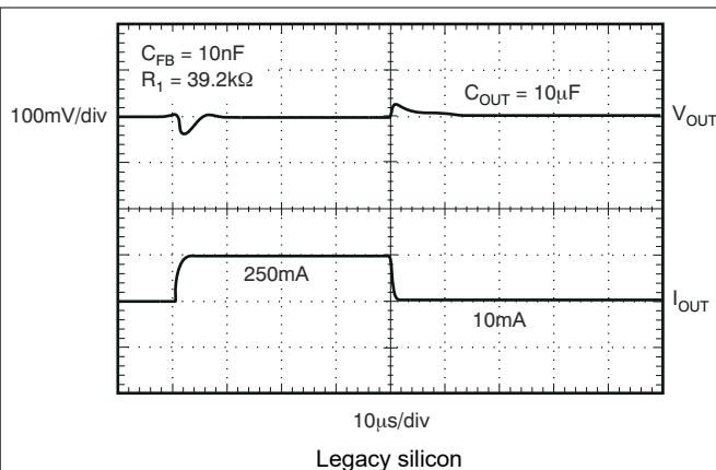
Figure 5-41. TPS73701 Load Transient, Adjustable Version
