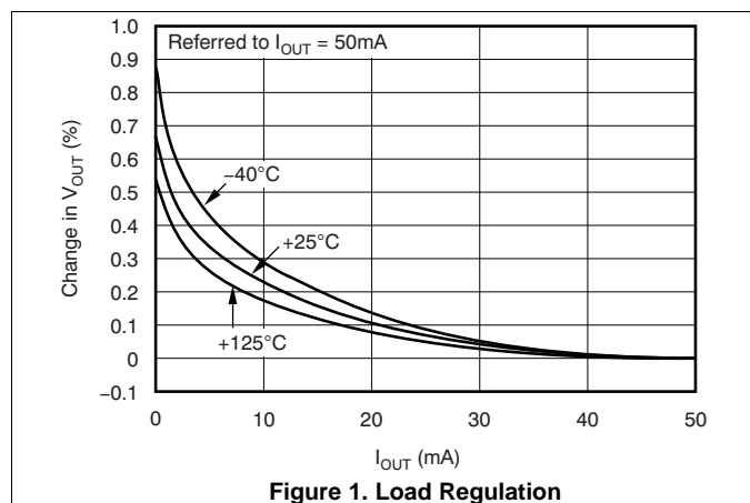
Figure 1. Load Regulation
