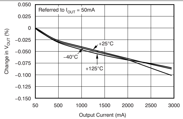
Figure 2. Load Regulation
