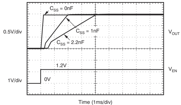
Turn-On Response
