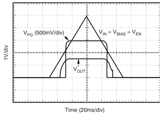
Figure 8-7. Power-Up, Power-Down
