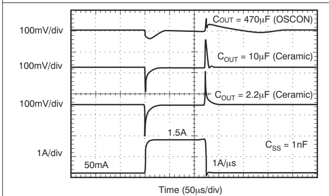
Figure 8-5. Output Load Transient Response
