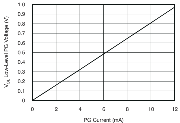
Figure 6-16. Low-Level PG Voltage vs Current
