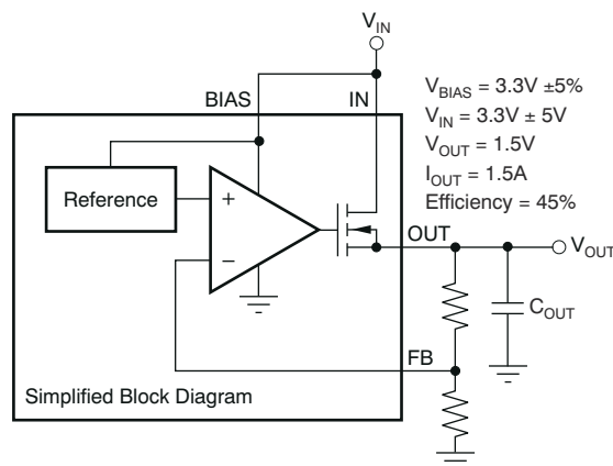
Figure 8-2. Typical Application of the TPS74901 Without an Auxiliary Bias
