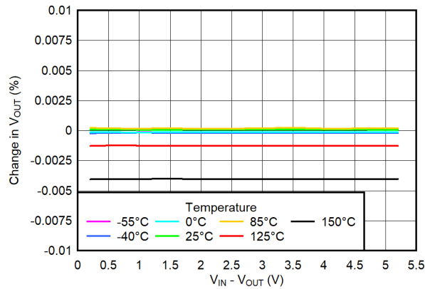
Figure 6-23. V_{IN} Line Regulation
