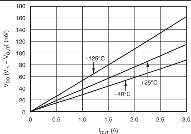
Figure 6-5. V_{IN} Dropout Voltage vs I_{OUT} and Temperature ( T_J )
