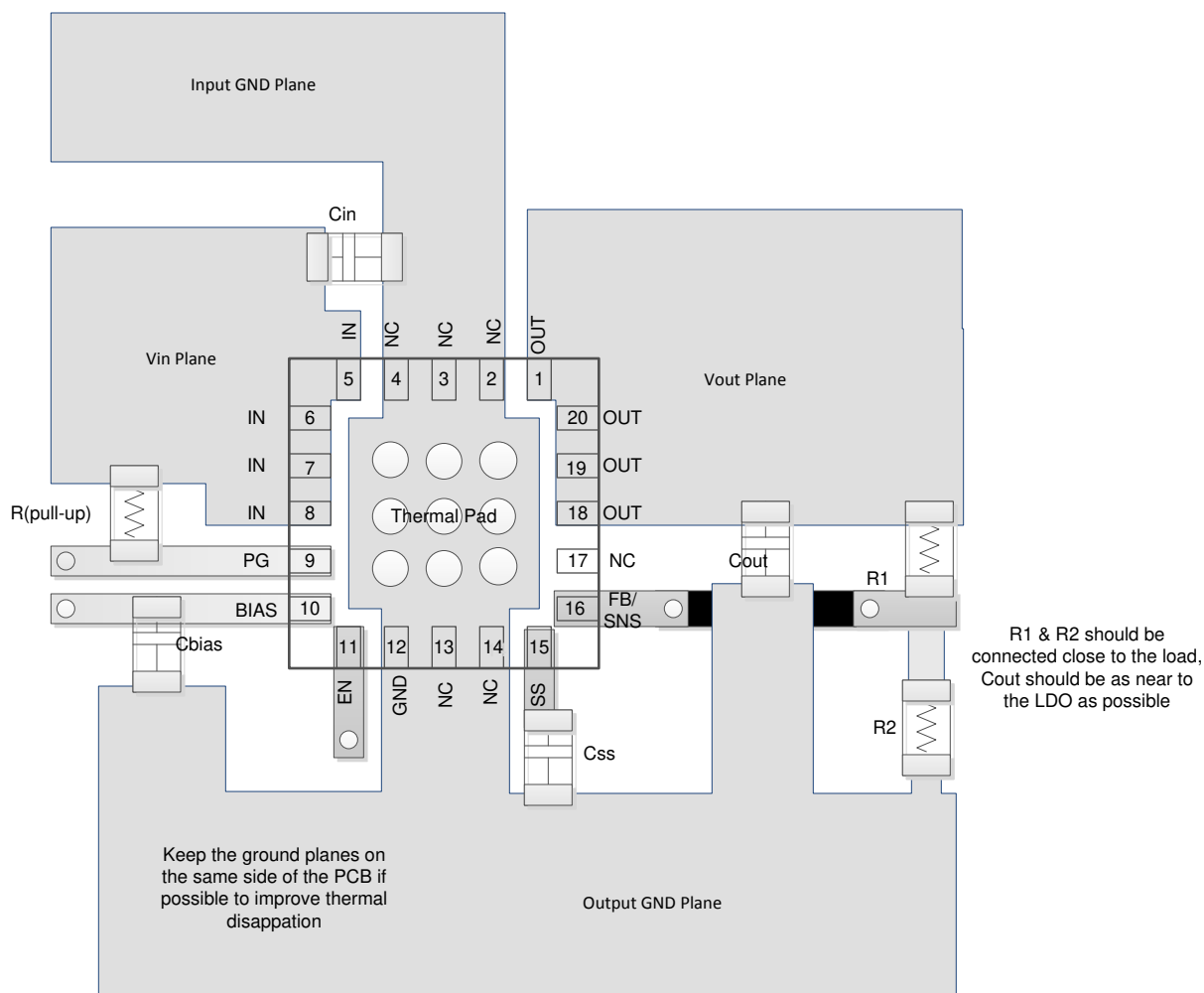
Figure 8-10. Layout Schematic (RGW Package)
