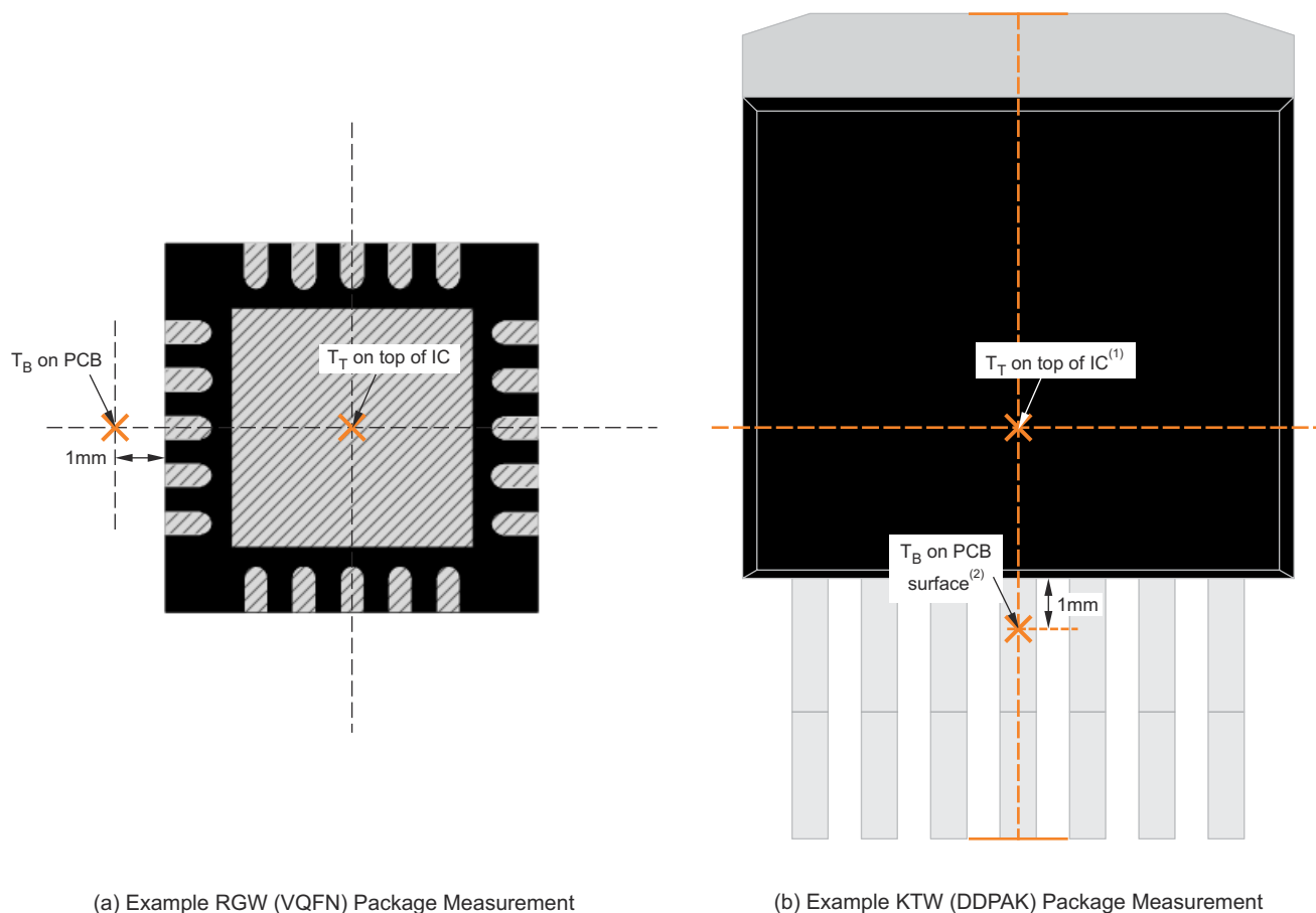
Figure 8-8. Measuring Points for T_T and T_B
