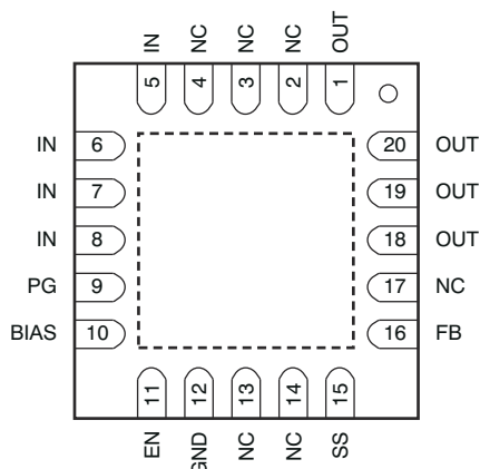
Figure 5-1. RGW Package, 20-Pin VQFN (Top View)
