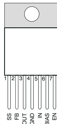
Figure 5-2. KTW Package, 7-Pin DDPAK/TO-263 (Top View)
