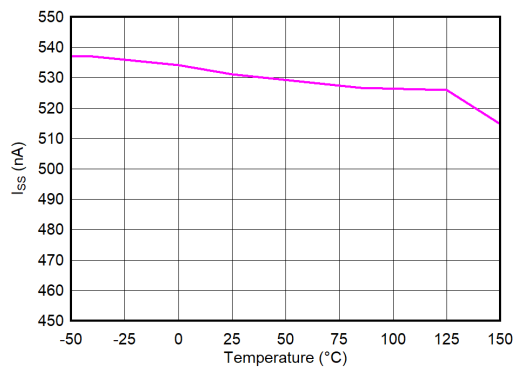
Figure 6-39. Soft-Start Charging Current ( I_{SS} ) vs Temperature ( T_J )
