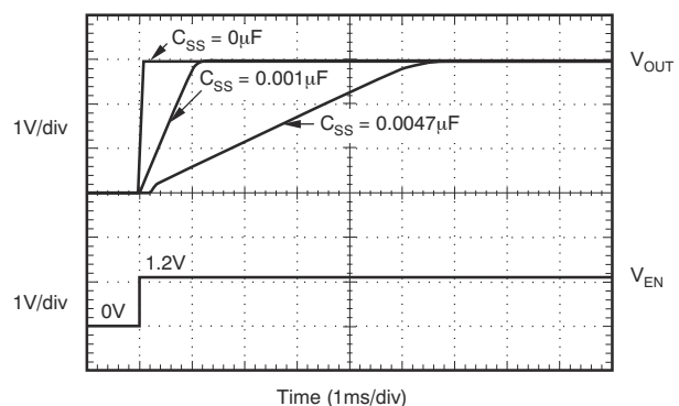
Turn-On Response
