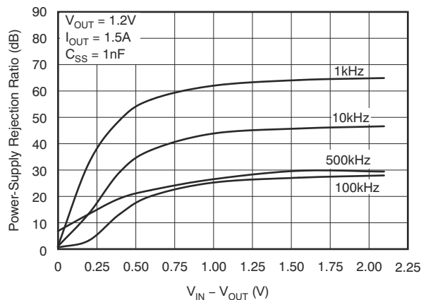
Figure 8-5. V_{IN} PSRR vs (V_{IN} - V_{OUT})
