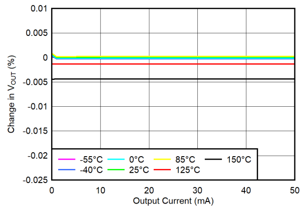
Figure 6-26. Load Regulation at Light Load
