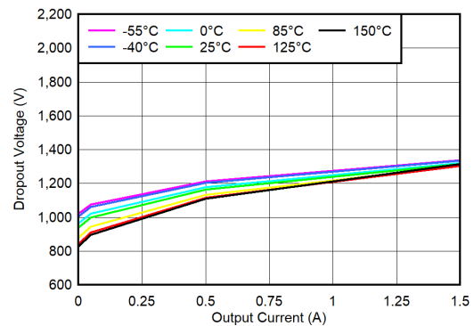
Figure 6-32. V_{BIAS} Dropout Voltage vs I_{OUT} and Temperature ( T_J )
