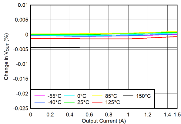
Figure 6-25. Load Regulation
