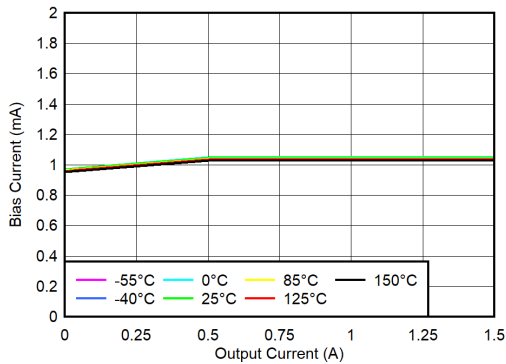
Figure 6-37. BIAS Pin Current vs Output Current and Temperature ( T_J )
