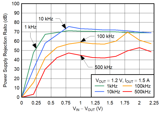
Figure 6-35. V_{IN} PSRR vs (V_{IN} - V_{OUT})
