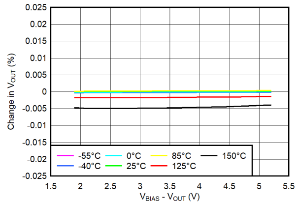
Figure 6-24. V_{BIAS} Line Regulation
