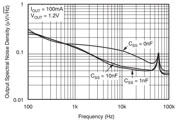
Figure 28. Noise Spectral Density
