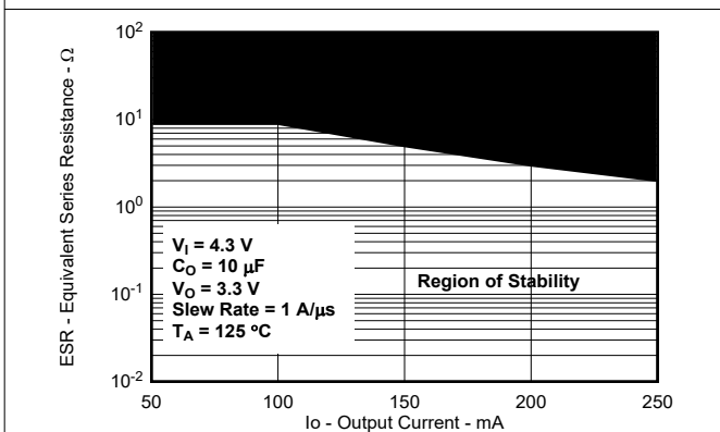
Figure 5-55. Typical Region of Stability ESR vs Output Current (New Chip)
