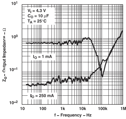
Figure 5-32. TPS76633 Output Impedance vs Frequency (Legacy Chip)
