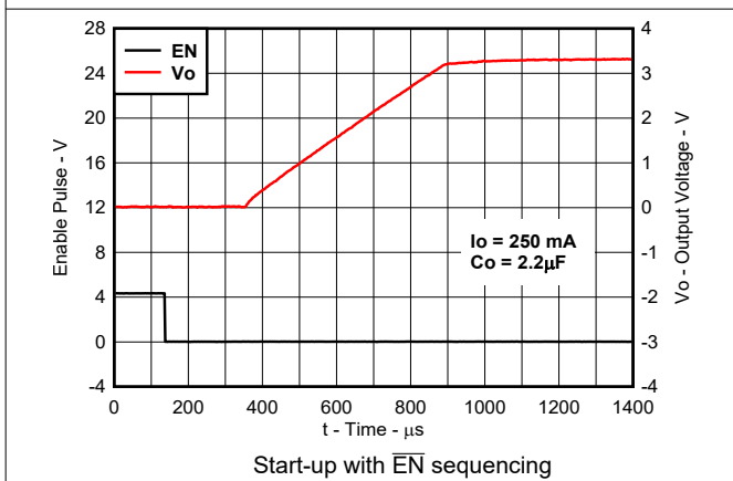
Figure 5-42. TPS76633 Output Voltage vs Time (New Chip)
