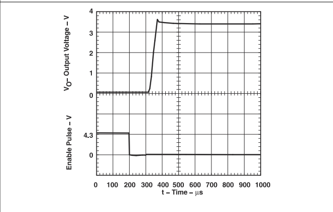
Figure 5-41. TPS76633 Output Voltage vs Time (Legacy Chip)
