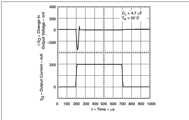
Figure 5-38. TPS76633 Load Transient Response (Legacy Chip)
