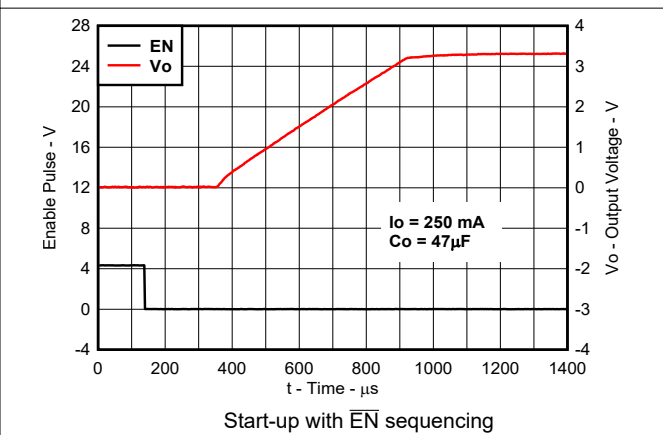
Figure 5-43. TPS76633 Output Voltage vs Time (New Chip)
