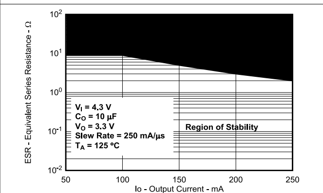
Figure 5-56. Typical Region of Stability ESR vs Output Current (Legacy Chip)
