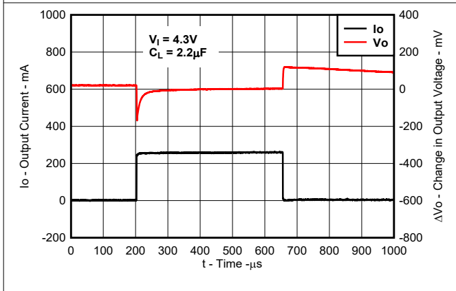
Figure 5-40. TPS76633 Load Transient Response (New Chip)
