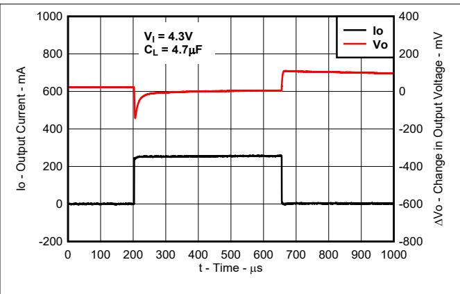
Figure 5-39. TPS76633 Load Transient Response (New Chip)
