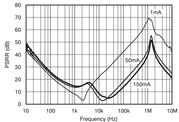
Figure 58. TPS78001 Ripple Rejection vs Frequency
