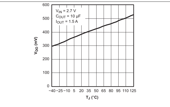
Figure 8. TPS78628 Dropout Voltage vs Junction Temperature
