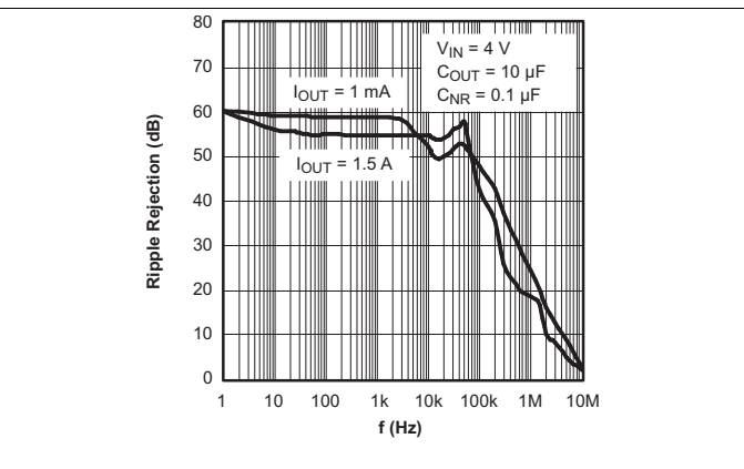
Figure 10. TPS78630 Ripple Rejection vs Frequency
