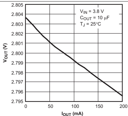
Figure 1. TPS79328 Output Voltage vs Output Current
