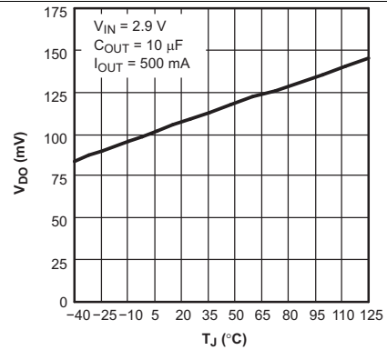
Figure 8. TPS79530 Dropout Voltage vs Junction Temperature
