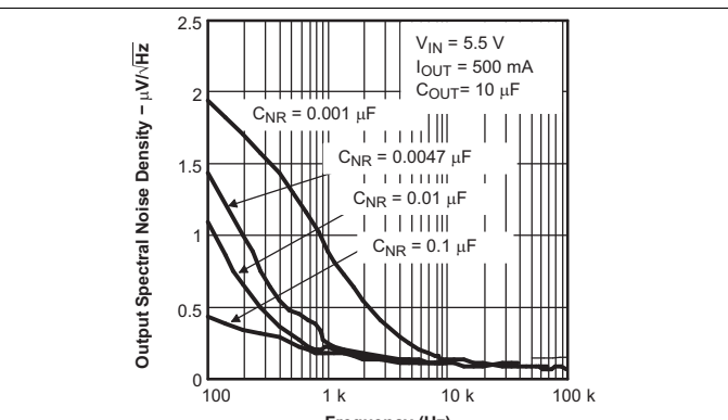
Figure 4. TPS79530 Output Spectral Noise Density vs Frequency
