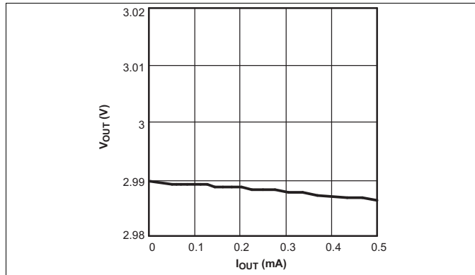
Figure 1. TPS79530 Output Voltage vs Output Current
