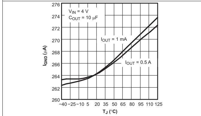
Figure 3. TPS79530 Ground Current vs Junction Temperature
