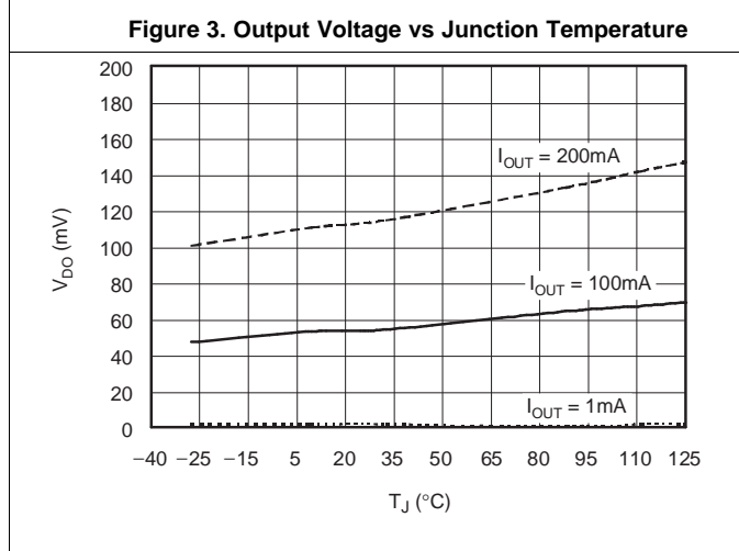
Figure 3. Output Voltage vs Junction Temperature
