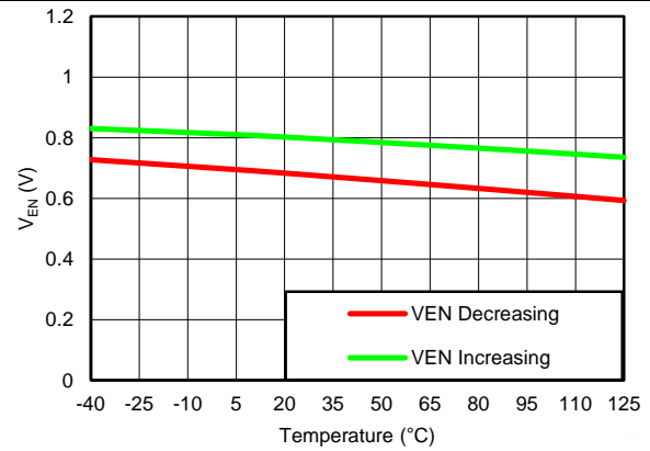
V_{OUT(TARGET)} = 0.8\text{ V} , V_{IN} = 1.4\text{ V} , V_{BIAS} = \text{Open} Figure 32. Minimum ANY-OUT V_{OUT} , Minimum V_{IN} , No BIAS Enable Threshold vs Temperature
