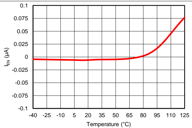
V_{OUT(TARGET)} = 0.8\text{ V} , V_{IN} = V_{EN} = 6.5\text{ V} , V_{BIAS} = \text{Open} Figure 34. Minimum ANY-OUT V_{OUT} , Maximum V_{IN} Enable Current vs Temperature
