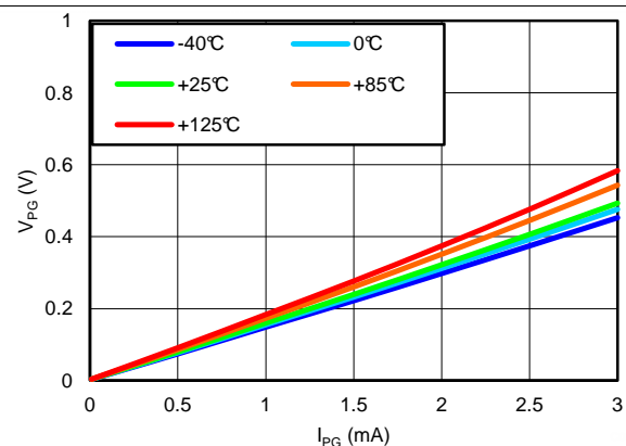
V_{OUT(TARGET)} = 0.8\text{ V} , V_{IN} = 1.4\text{ V} , V_{BIAS} = \text{Open} Figure 36. Minimum ANY-OUT V_{OUT} , Minimum V_{IN} , No BIAS PG Low Voltage vs PG Current
