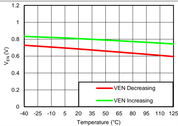
V_{OUT(TARGET)} = 0.8\text{ V} , V_{IN} = 6.5\text{ V} , V_{BIAS} = \text{Open} Figure 33. Minimum ANY-OUT V_{OUT} , Maximum V_{IN} Enable Threshold vs Temperature
