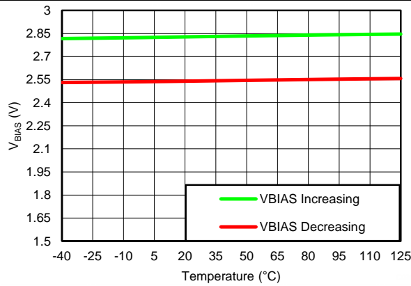
V_{OUT(TARGET)} = 0.8\text{ V} , V_{IN} = 1.1\text{ V} Figure 31. Minimum ANY-OUT V_{OUT} , Minimum V_{IN} BIAS UVLO Threshold vs Temperature
