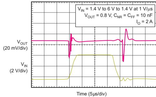
Figure 49. Line Transient
