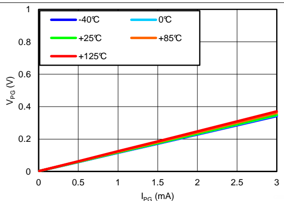
V_{IN} = 6.5\text{ V} , V_{OUT(TARGET)} = 0.8\text{ V} , V_{BIAS} = \text{Open} Figure 35. Minimum ANY-OUT V_{OUT} , Maximum V_{IN} , No BIAS PG Low Voltage vs PG Current
