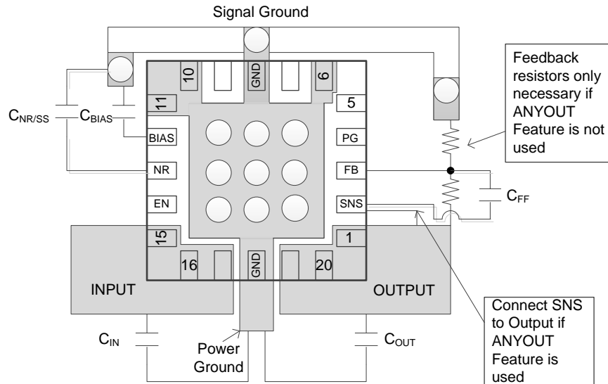
Figure 57. Example Layout
