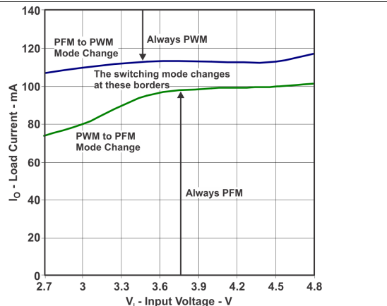
Figure 40. PFM/PWM Boundaries
