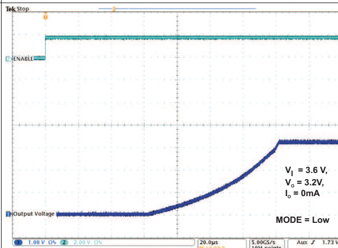
Figure 24. TPS82699 Start-Up
