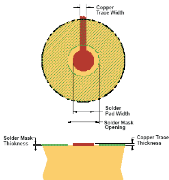
Figure 45. Recommended Land Pattern Image And Dimensions
