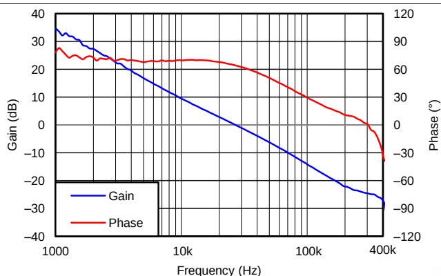
Figure 10. V OUT = 1.8 V, I OUT = 10 A, C OUT1 = 200 \mu F ceramic, f sw = 500 kHz
