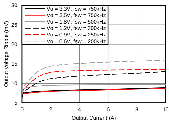
Figure 8. Voltage Ripple vs. Output Current
