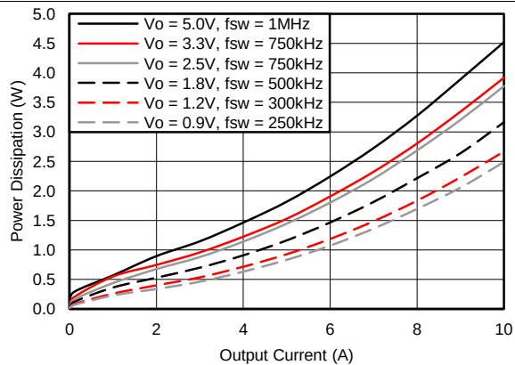
Figure 3. Power Dissipation vs. Output Current
