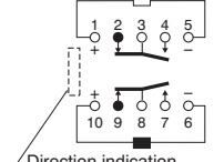
2-coil latching
