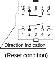
2-coil latching
