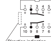
2-coil latching
