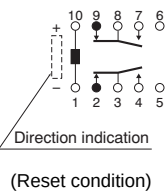
1-coil latching
