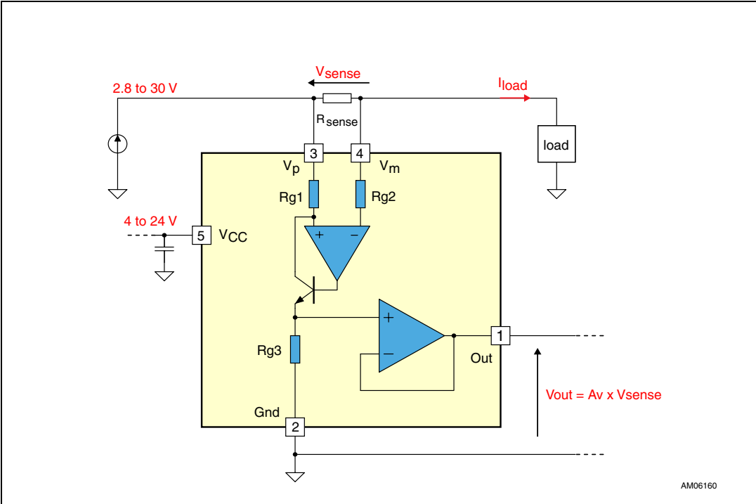
Figure 1. Application schematics
