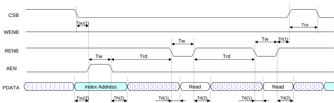
Fig 61 Read timing of parallel interface with auto index increment mode
