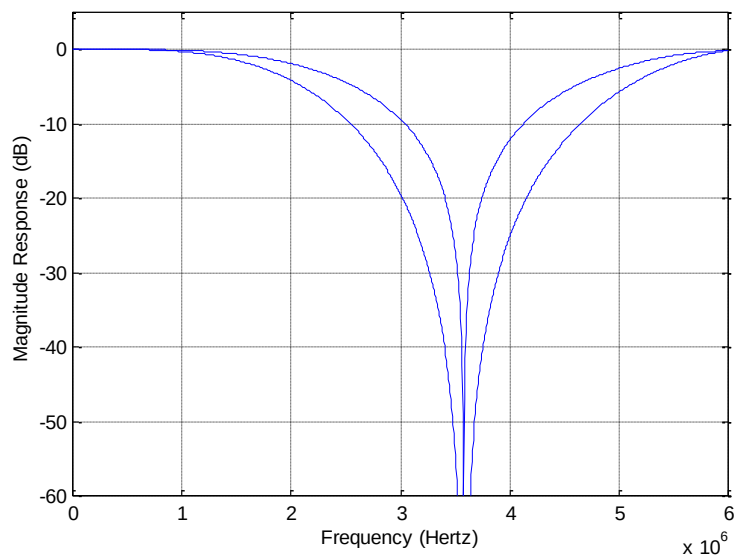
Fig 3 The frequency response of luminance notch filter for NTSC
