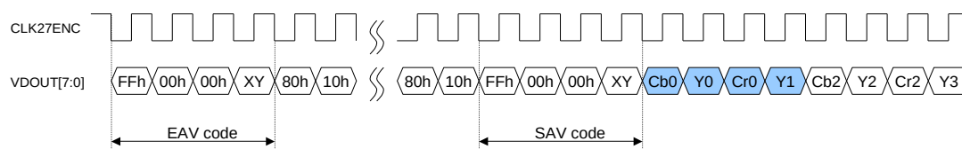
Fig 49 Timing diagram of single output mode
