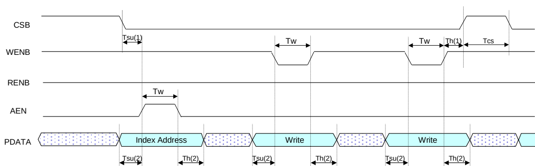
Fig 60 Write timing of parallel interface with auto index increment mode
