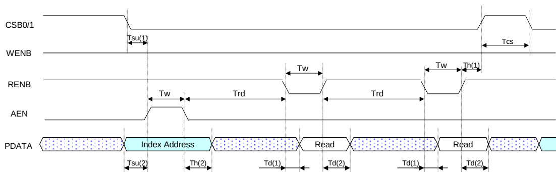
Fig 56 Read timing of parallel interface with auto index increment mode
