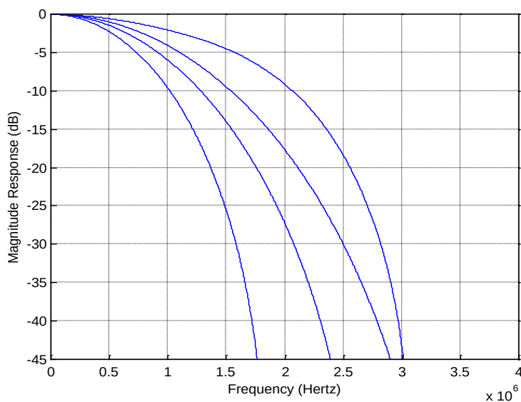
Fig 6 The frequency response of chrominance LPF
