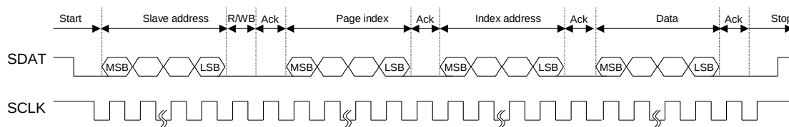
Fig 53 Write timing of serial interface
