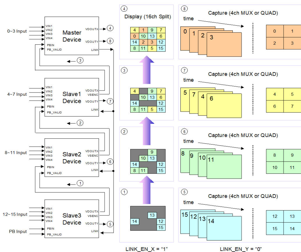
Fig 30 Cascade connection with X path only
