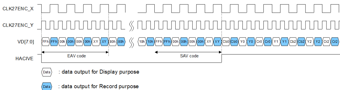
Fig 50 Timing diagram of dual output mode
