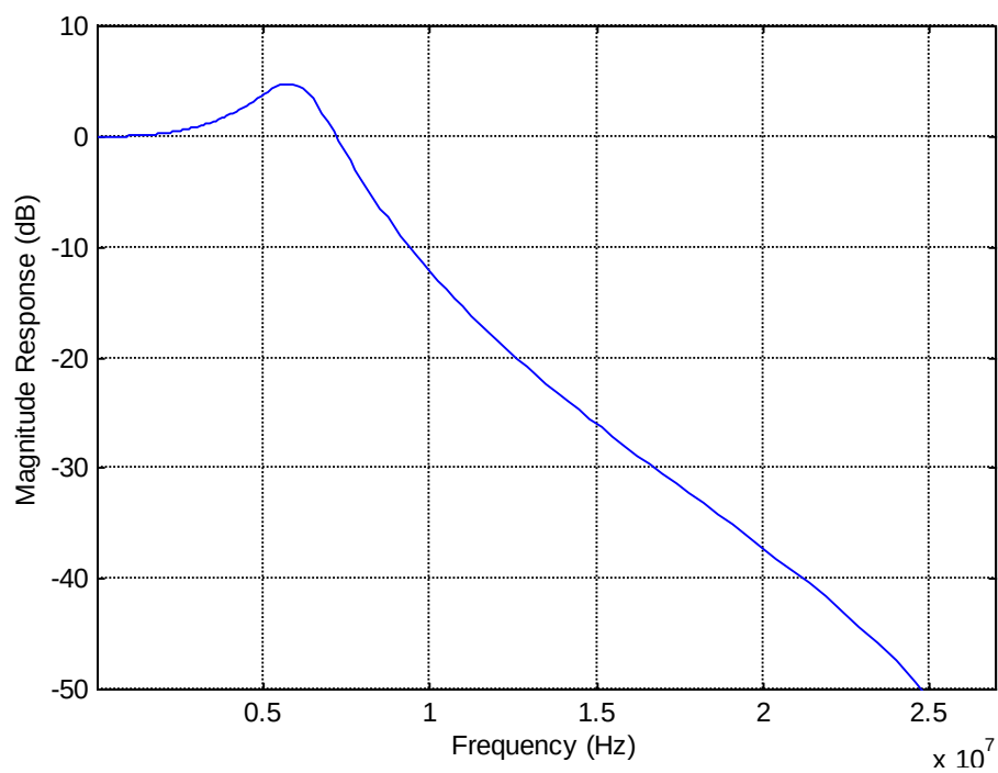
Fig 48 Frequency response of reconstruction filter
