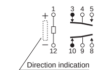
Schematic (Bottom view) Single side stable
