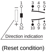
Schematic (Bottom view) Single side stable 1 coil latching
