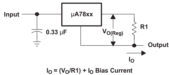
Figure 8. Current Regulator
