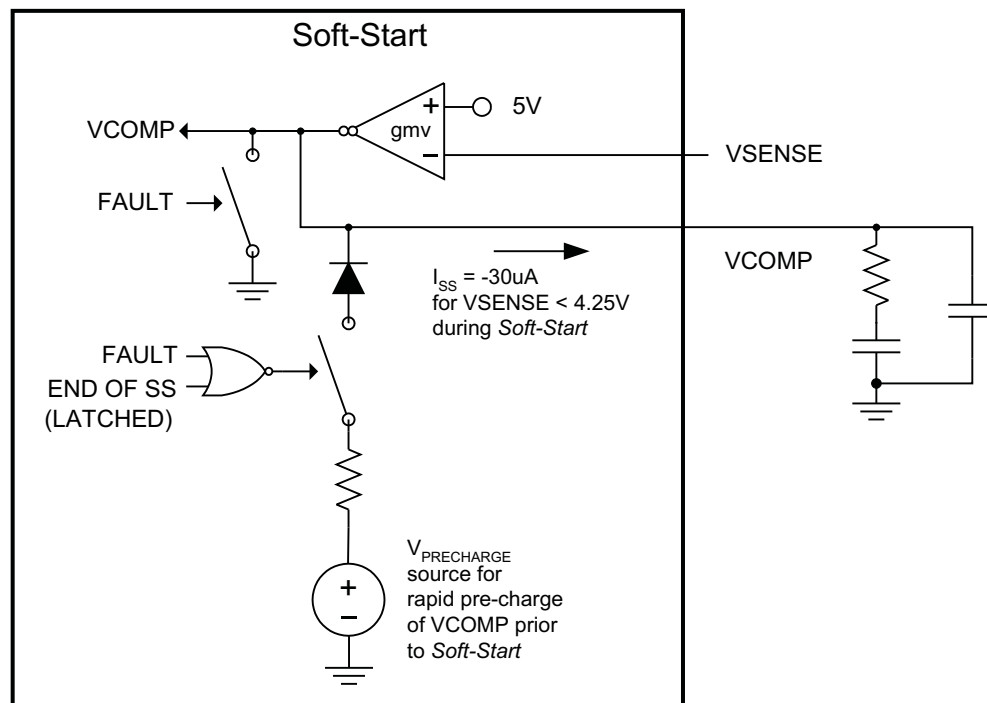
Figure 18. Soft Start
