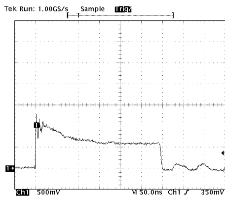
ESD Clamping (+8kV Contact)
