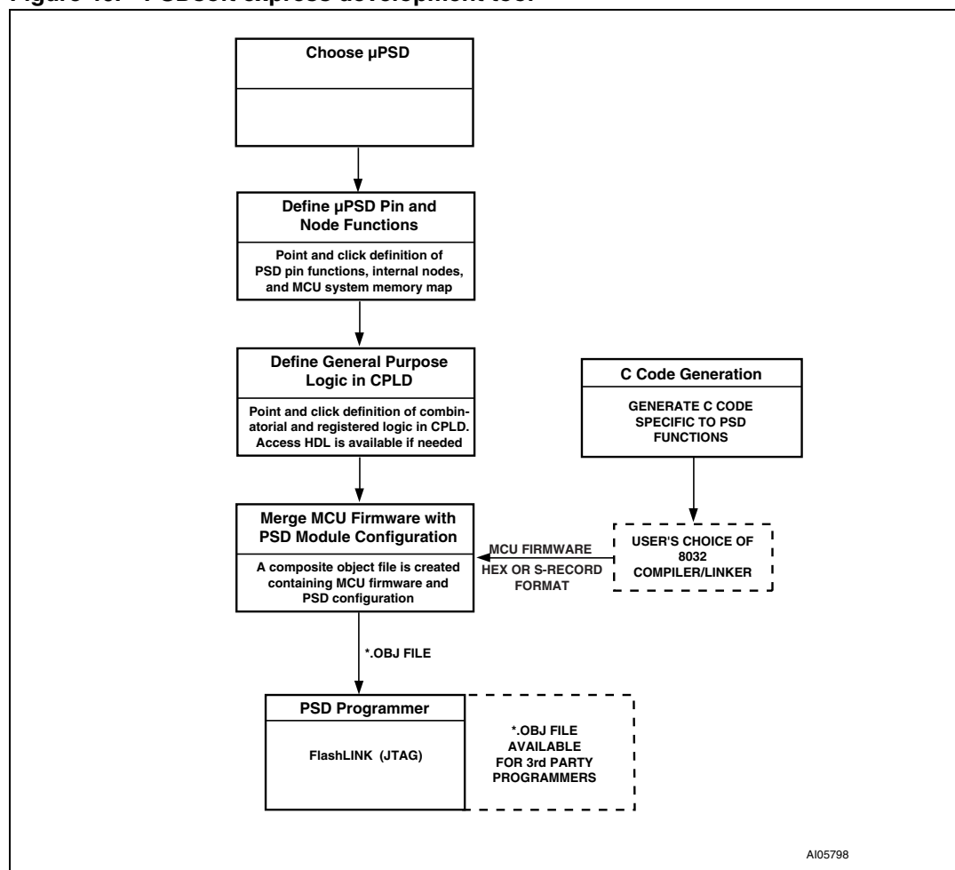
Figure 46. PSDsoft express development tool
