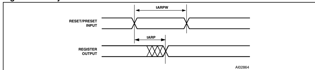
Figure 74. Asynchronous \overline{\text{Reset}} / Preset
