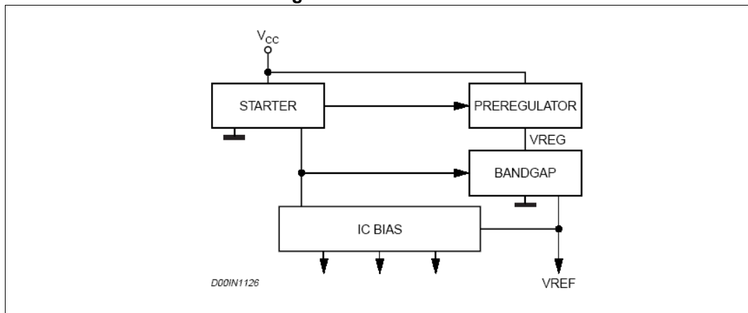
Figure 4. Internal circuit
