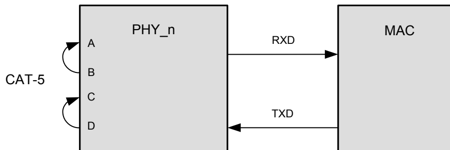
Figure 23. Connector Loopback
